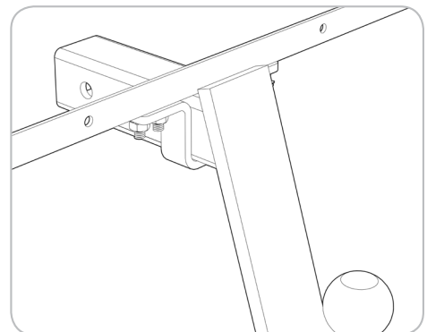
Assembled hitch insert bracket and support bar.
