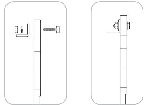
Side View: Installing the DuallyGuard to the support Bar using the set of 12, 1/4"-20-1" nuts and 1/4 washers and bolts.
