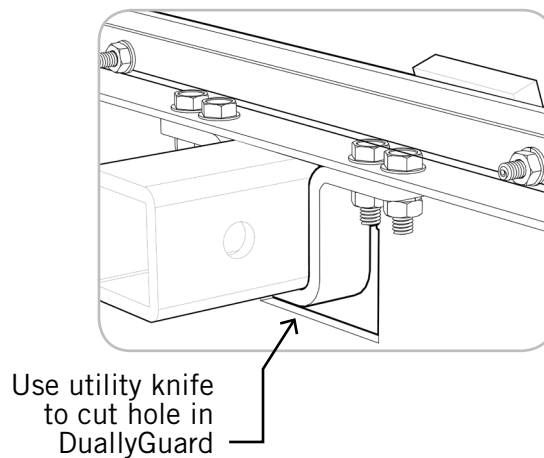
Assembled hitch insert bracket and support bar.
